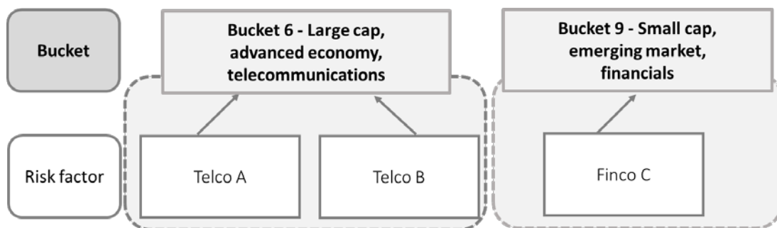
Graph A2: Step 3 – Aggregation of risk-weighted sensitivities within buckets
