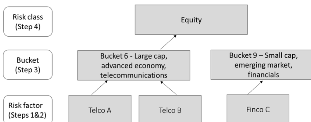
Graph A1: Steps for delta risk capital requirement
