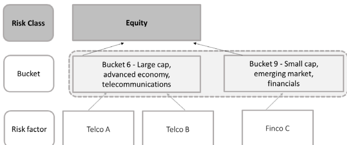
Graph A3: Step 3 – Aggregation of risk-weighted sensitivities across buckets
